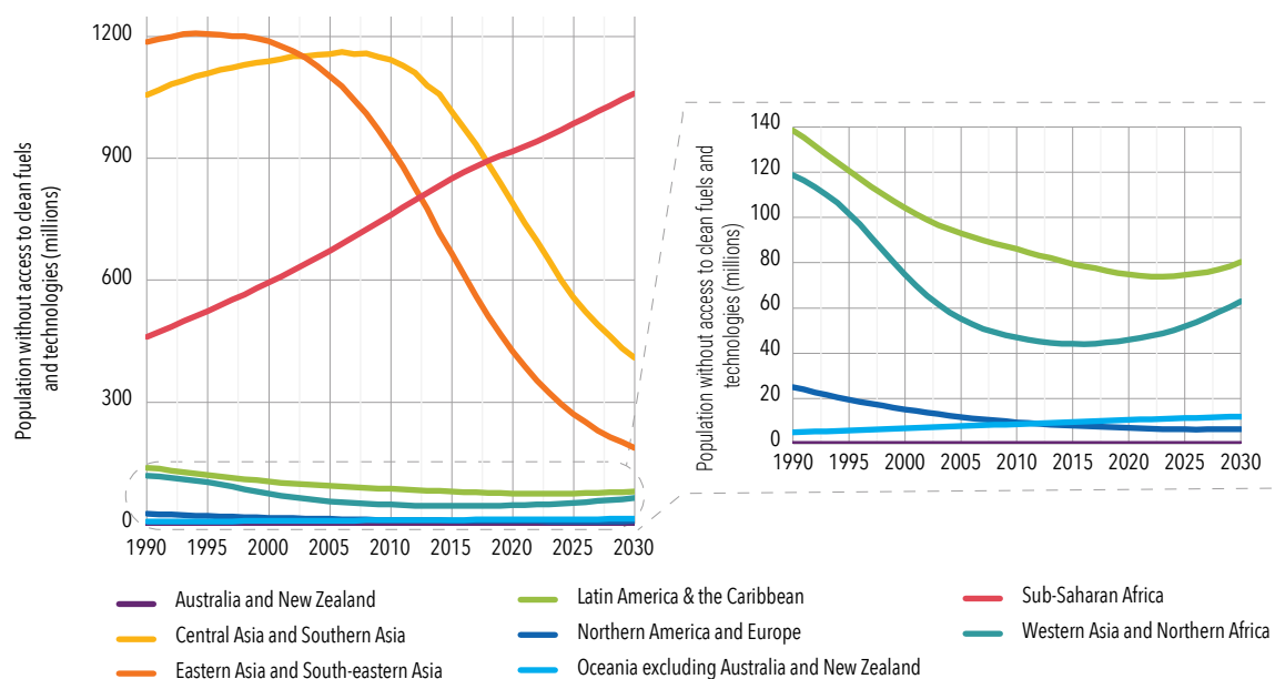
FIGURE 2.6 • NUMBER OF PEOPLE WITHOUT ACCESS TO CLEAN FUELS AND TECHNOLOGIES, BY REGION, 1990-2030
